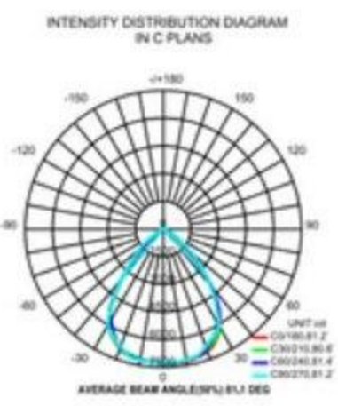
100W-Light Distribution Curve
